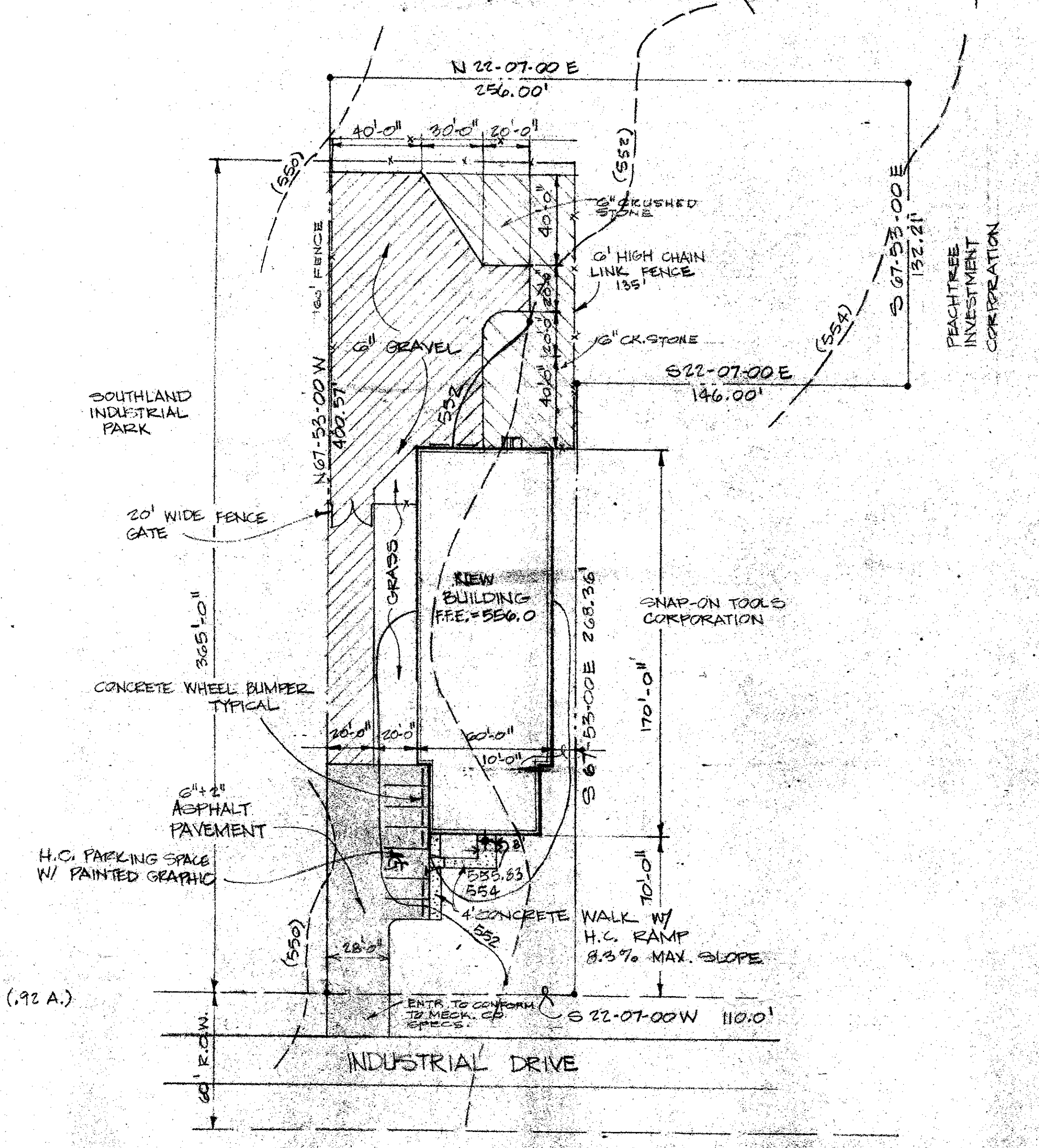
SITE PLAN 1" = 40'-0"
